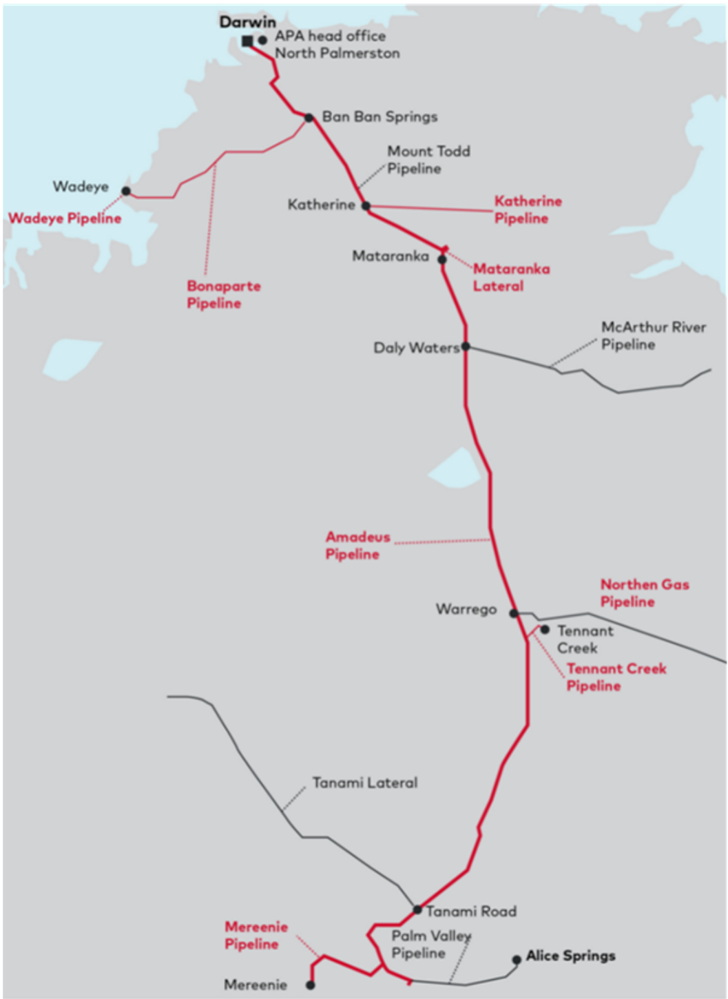
Exhibit 1: APA Group's Northern Territory pipeline network
